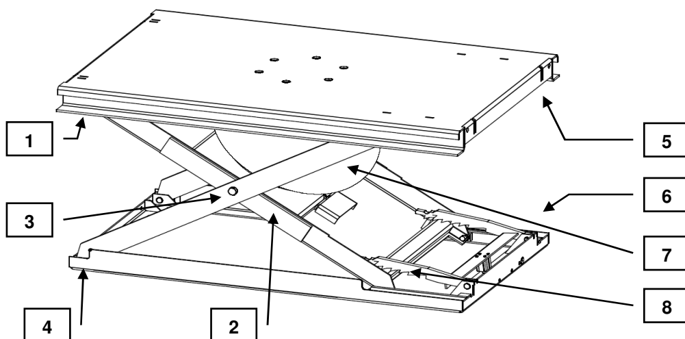
Diagram 8: Lubrication and test points
