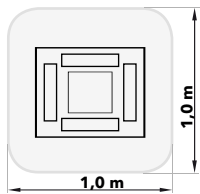
IRT COMBI 4-1 IR-UVA One cassette at a distance of 550 mm with an UV-A intensity of 25mW/cm 2 .
