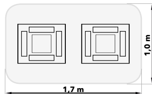
IRT COMBI 4-2 IR-UVA Two cassettes at a distance of 550 mm with an UV-A intensity of 25mW/cm 2 .
