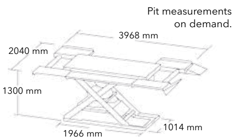
For wheel bases up to 3500 mm
