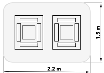
IRT COMBI 4-2 IR-UVA Two cassettes at a distance of 600 mm, on black sheet metal
